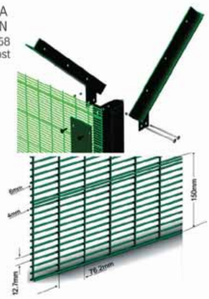
PRISON FENCE Bowed fence with circular hollow section post
